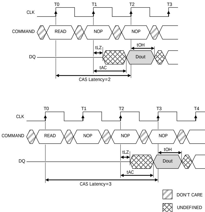
Figure7: CAS Latency
